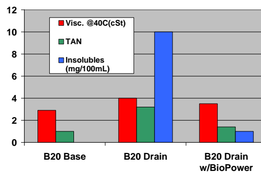
Figure 3. Reduced Insolubles, Viscosity and TAN from Modified D2274 Test
